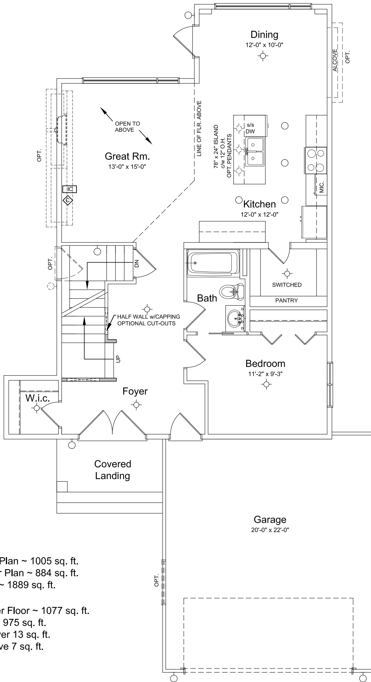
Main Floor Plan
