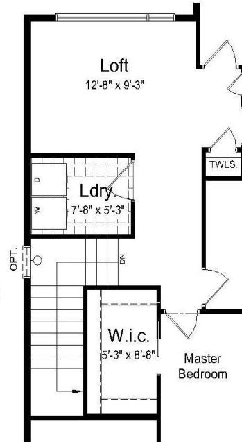
Upper Floor Plan w/Loft
