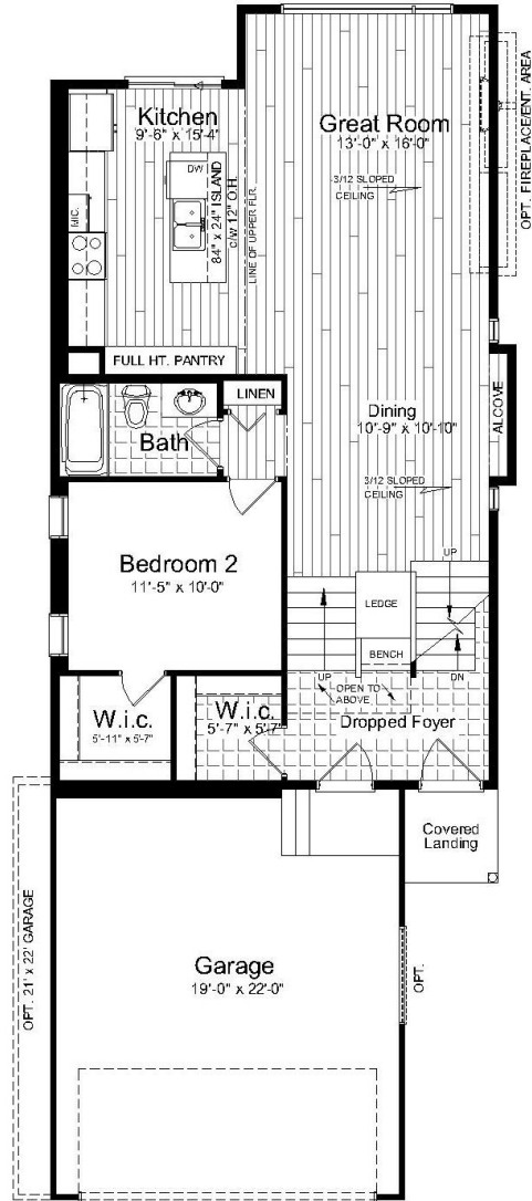
Upper Floor Plan 976 sq. ft.
