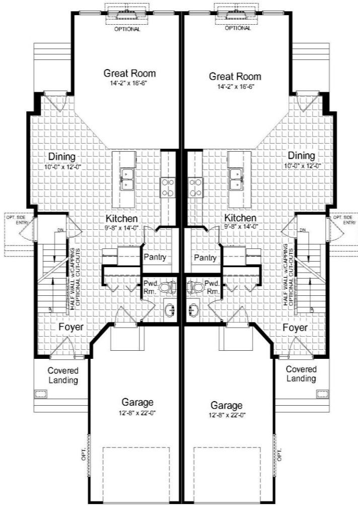
Main Floor Plan 777 Sq. ft. (ea. unit)
