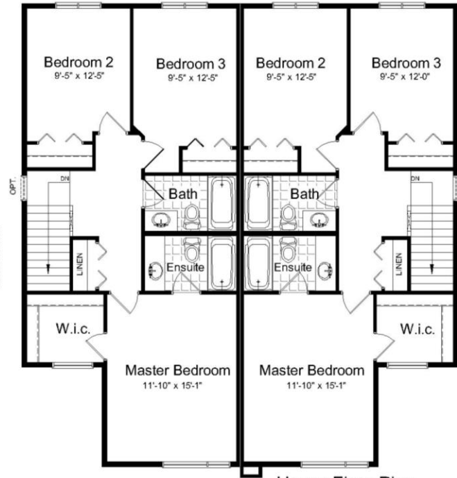
Upper Floor Plan 774 Sq. ft. (ea. unit)
