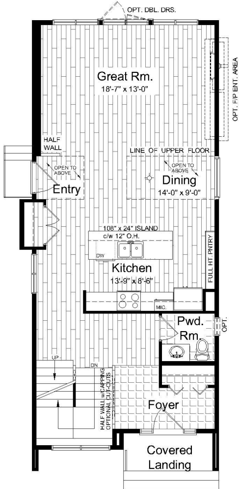
Main Floor Plan ~ 904 sq. ft.
