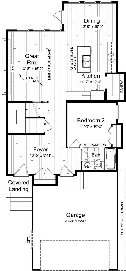
Main Floor Plan 993 sq. ft.
