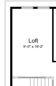
Upper Floor Plan w/Opt. Loft
