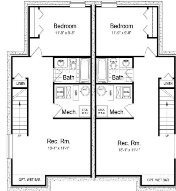
Optional Finished Bsmt. Layout 573 sq. ft. (finished space)
