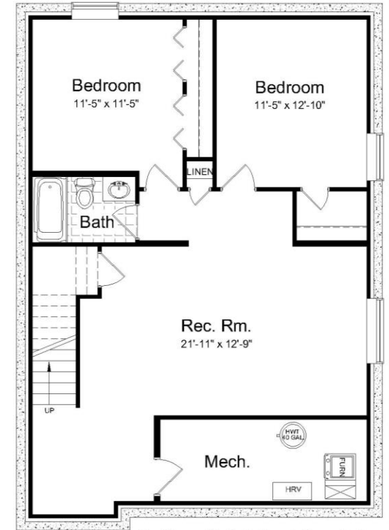
Optional Finished Bsmt. Layout 844 sq. ft. (finished space)
