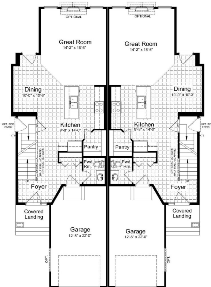
Main Floor Plan 777 Sq. ft. (ea. unit)
