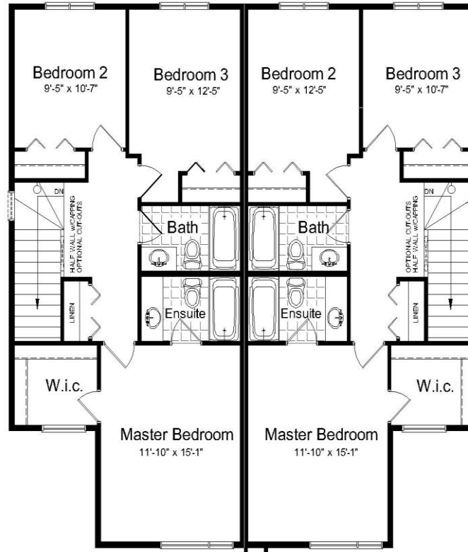
Upper Floor Plan 774 Sq. ft. (ea. unit)
