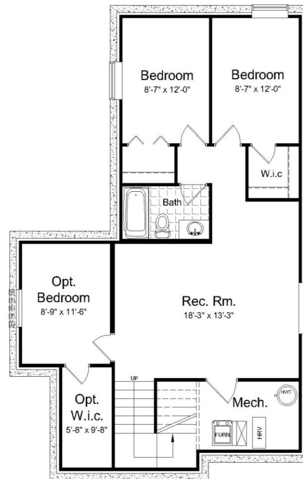
Optional Finished Bsmt. Layout 820 sq. ft. (finished space)
