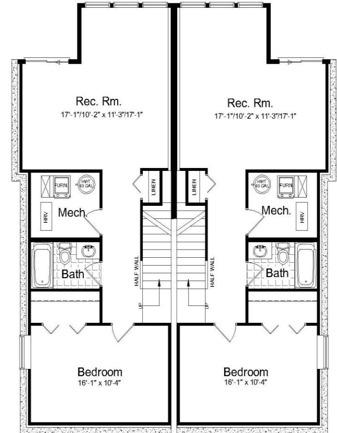
Optional Finished Bsmt. Layout 634 sq. ft. (finished space)
