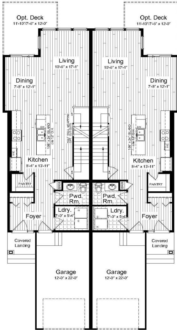
Main Floor Plan 801 sq. ft.
