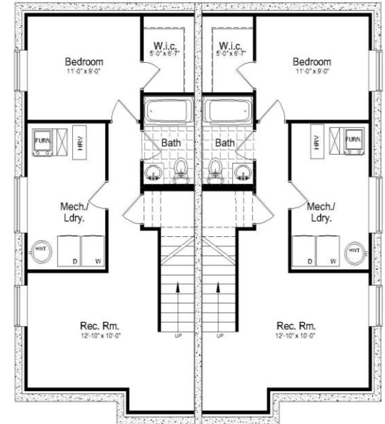
Optional Finished Bsmt. Layout 498 sq. ft. (finished space)
