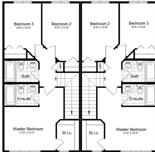
Main Floor Plan 630 sq. ft. ea. unit
