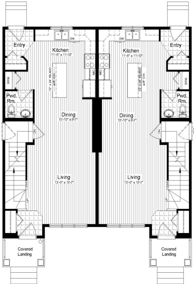
Main Floor Plan 646 sq. ft. ea. unit
