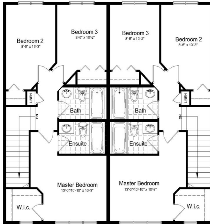
Main Floor Plan 630 sq. ft. ea. unit
