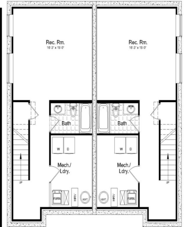
Optional Finished Bsmt. Layout 443 sq. ft. (finished space)
