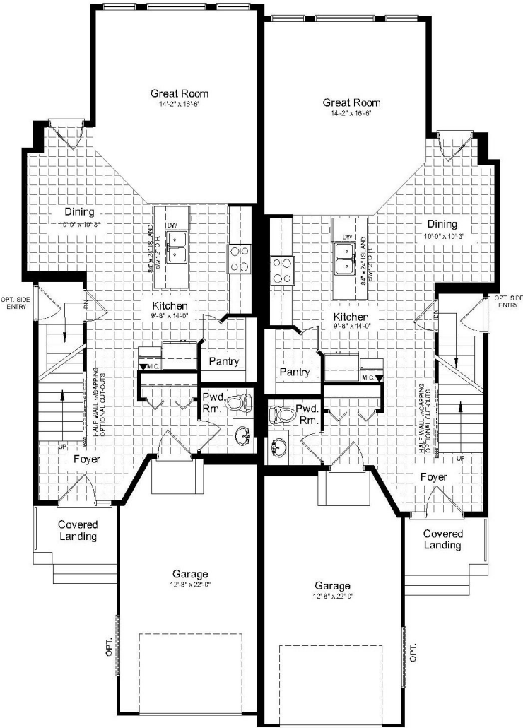
Main Floor Plan 777 Sq. ft. (ea. unit)
