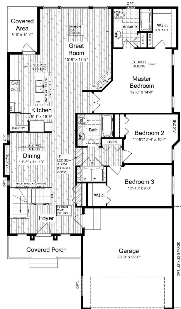
Main Floor Plan 1645 sq. ft.
