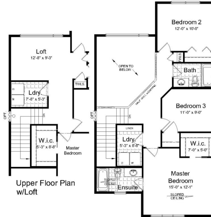
Upper Floor Plan 884 sq. ft.
