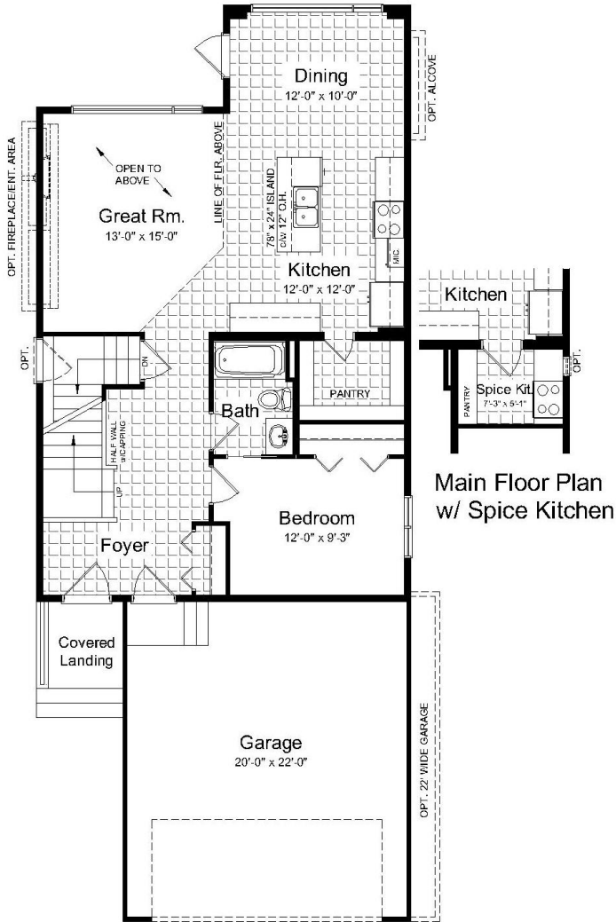
Main Floor Plan 975 sq. ft.
