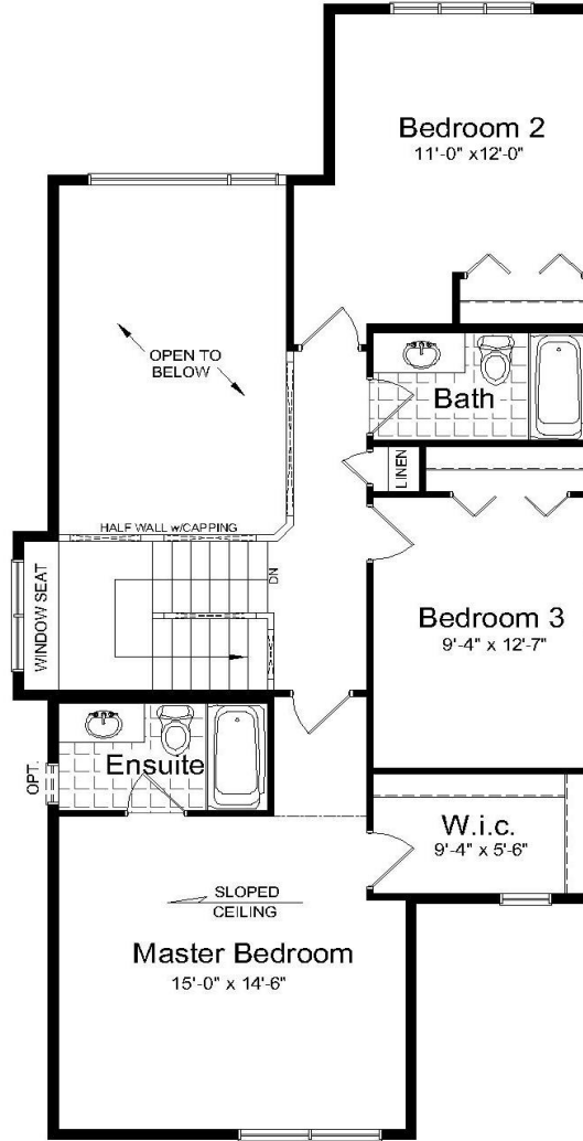
Upper Floor Plan 926 sq. ft.
