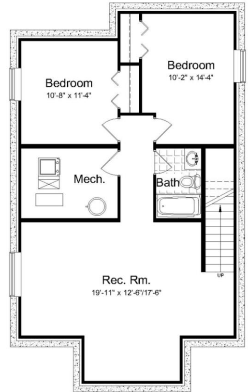
Optional Finished Bsmt. Layout 778 sq. ft. (finished space)
