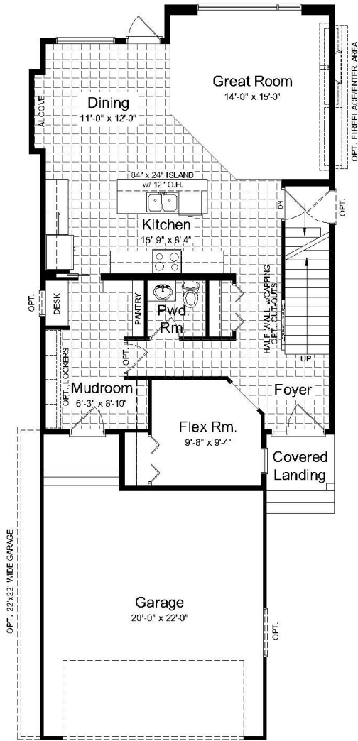
Main Floor Plan 1028 sq. ft.
