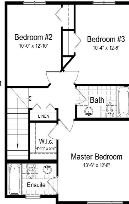
Upper Floor Plan 759 sq. ft.
