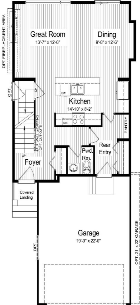
Main Floor Plan 737 sq. ft.
