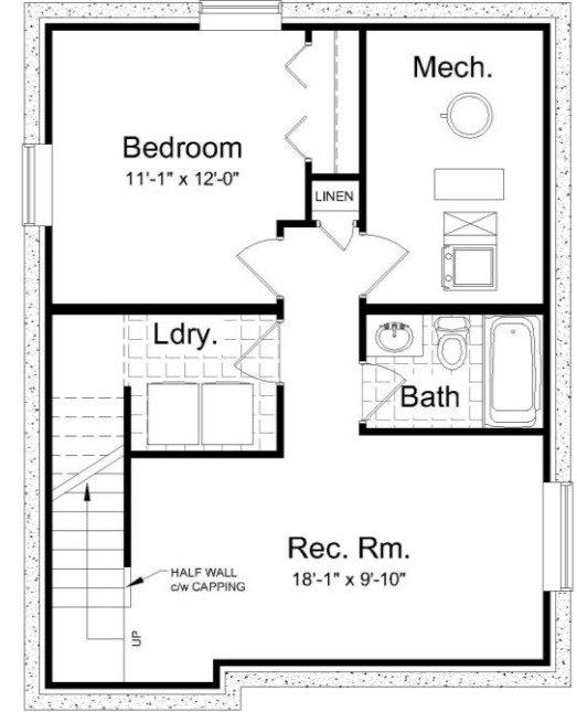
Optional Finished Bsmt. Layout 509 sq. ft. (finished space)
