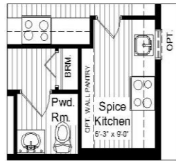
Opt. Main Floor Plan ~ w/Spice Kitchen
