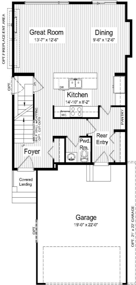
Main Floor Plan 737 sq. ft.
