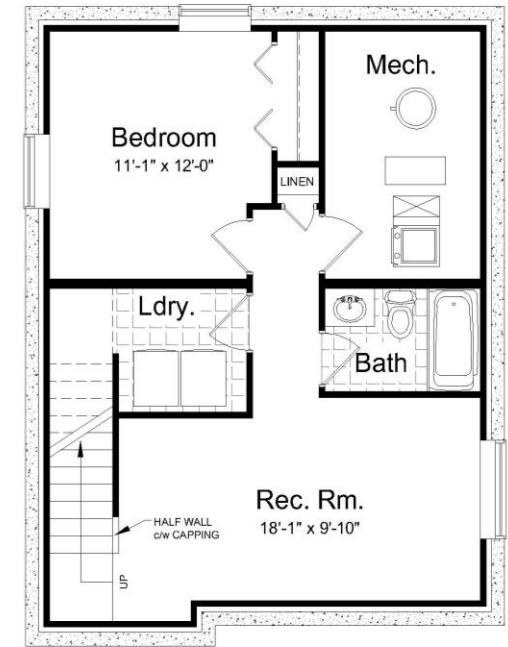
Optional Finished Bsmt. Layout 509 sq. ft. (finished space)
