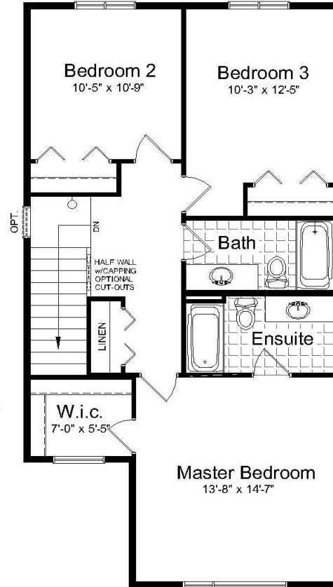
Upper Floor Plan ~ 858 sq. ft.
