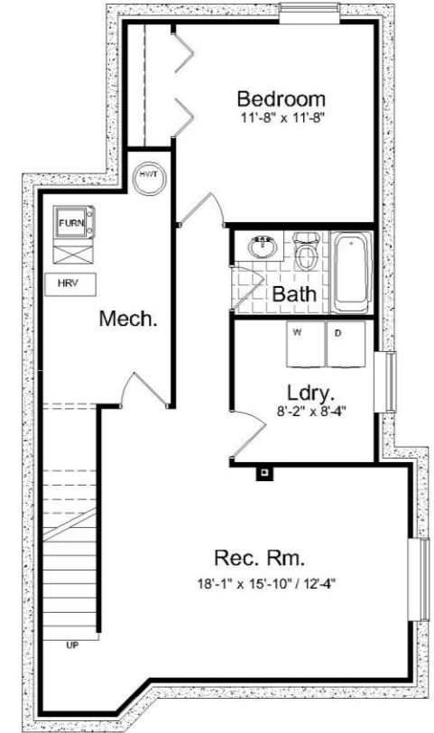
Optional Finished Bsmt. Layout 632 sq. ft. (finished space)
