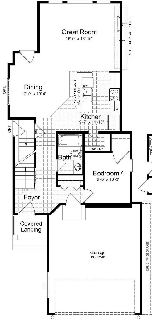
Main Floor Plan ~ 911 sq. ft.
