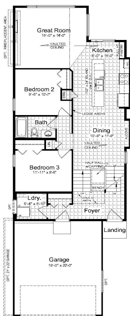
Main Floor Plan 1155 sq. ft.
