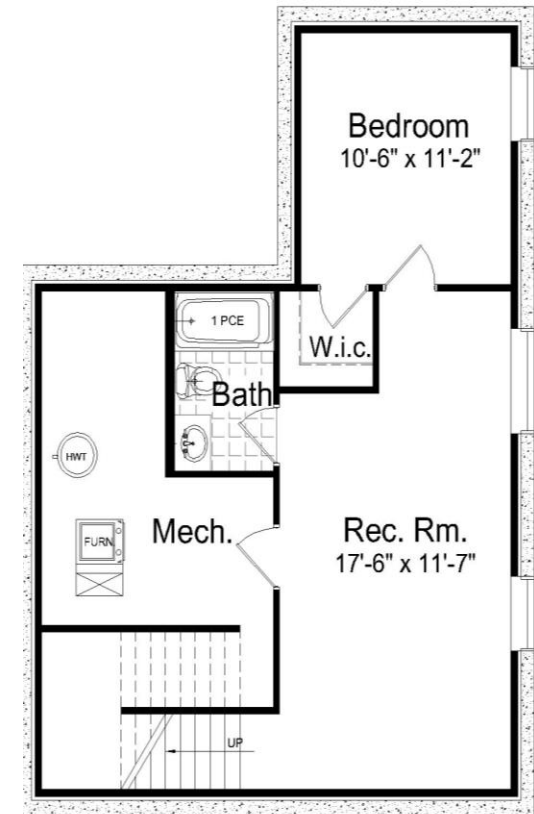
Optional Basement Layout 461 Sq. ft. (finished space)
