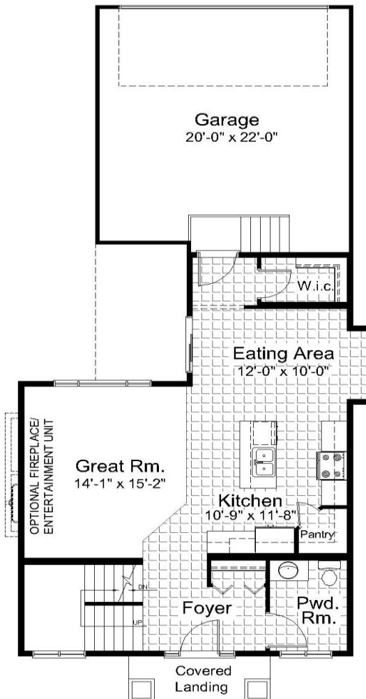
Main Floor Plan 796 Sq. ft.
