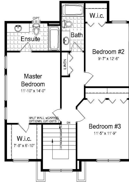
Upper Floor Plan 846 sq. ft.
