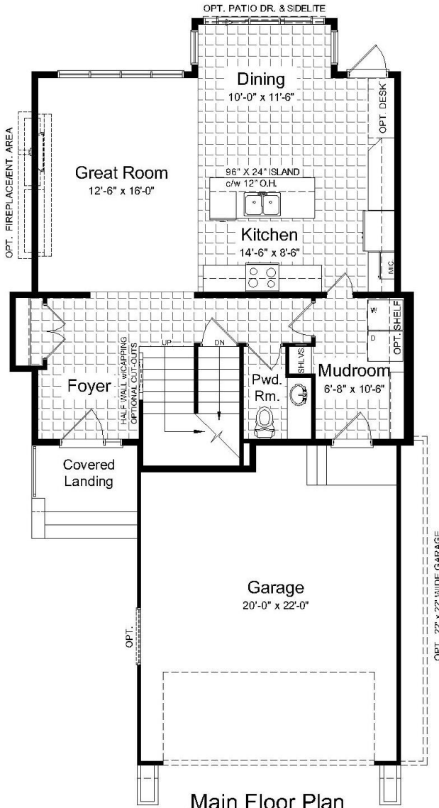
Main Floor Plan 867 sq. ft.
