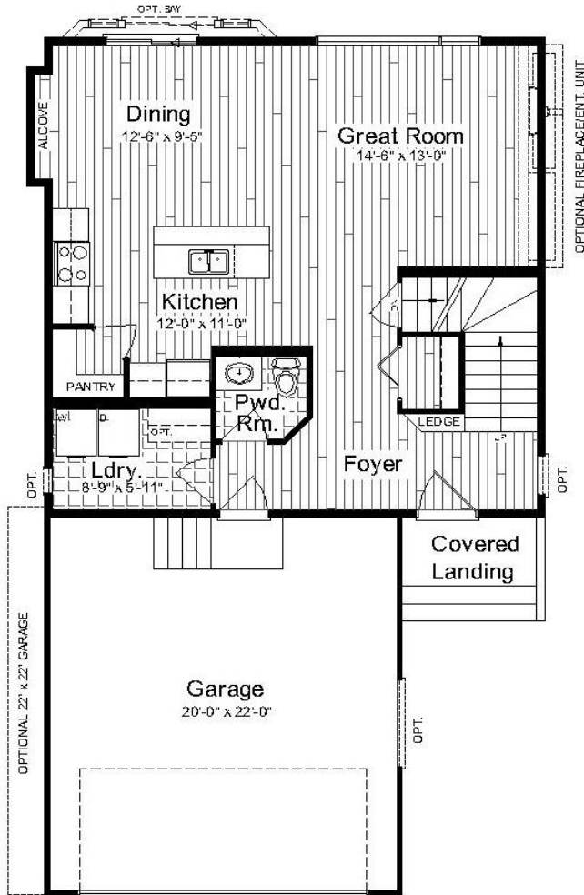
Main Floor Plan 791 sq. ft.
