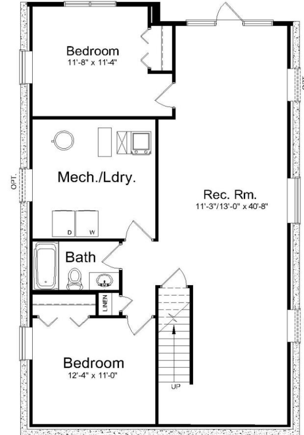
Optional Walk-out Basement Layout 923 Sq. ft. (finished space)
