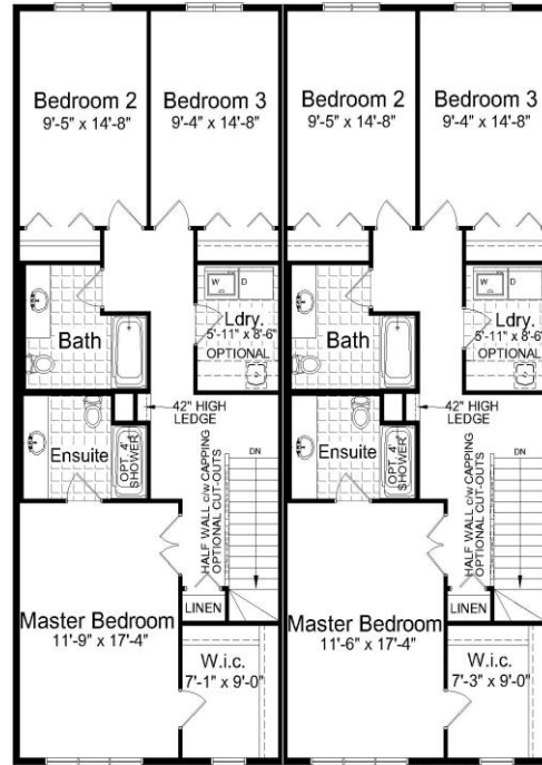
Upper Floor Plan 1040 Sq. ft. - ea. unit
