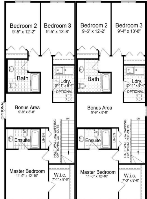
Optional Upper Floor Plan w/Bonus Rm. 1040 Sq. ft. - ea. unit
