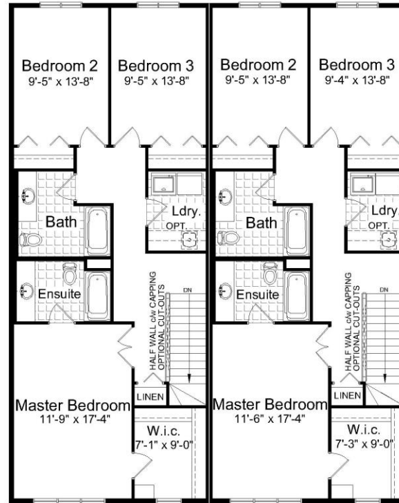
Upper Floor Plan 1000 Sq. ft. - ea. unit
