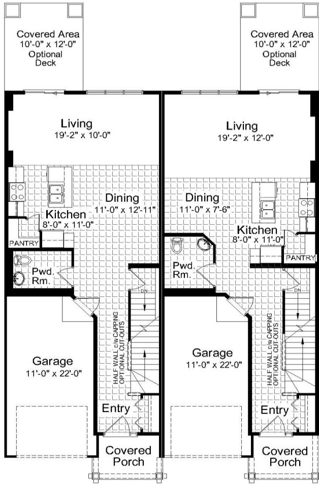
Main Floor Plan 733 Sq. ft. - ea. unit
