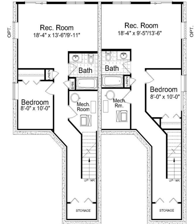
Optional WalkOut Bsmt. Layout 563 Sq. ft. ea. unit (finished space)
