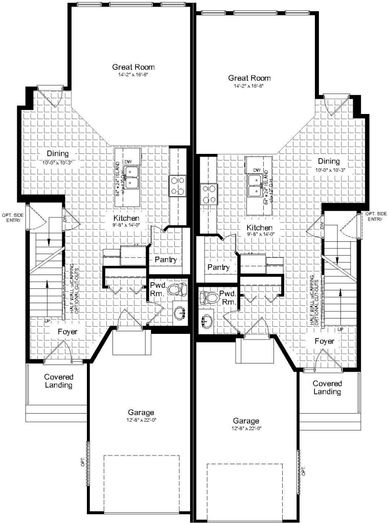
Main Floor Plan 777 Sq. ft. (ea. unit)
