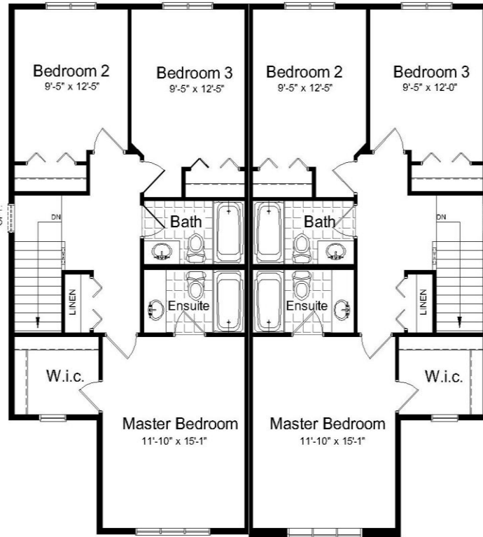
Upper Floor Plan 774 Sq. ft. (ea. unit)
