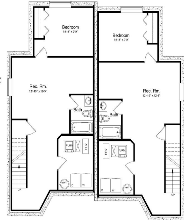
Optional Basement Layout 515 Sq. ft. (finished space ea. unit)
